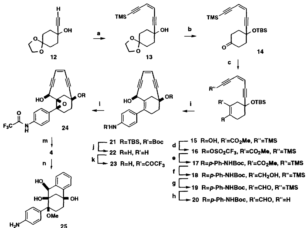
Scheme 3 a
